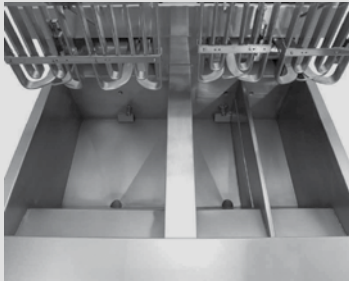
picture of open pot (FPEL214)
