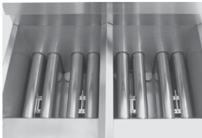
picture of tube frypot (HD60)
